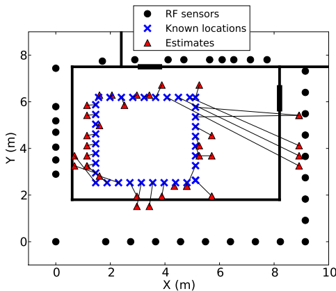
Fig. 7: Estimates from VRTI.
