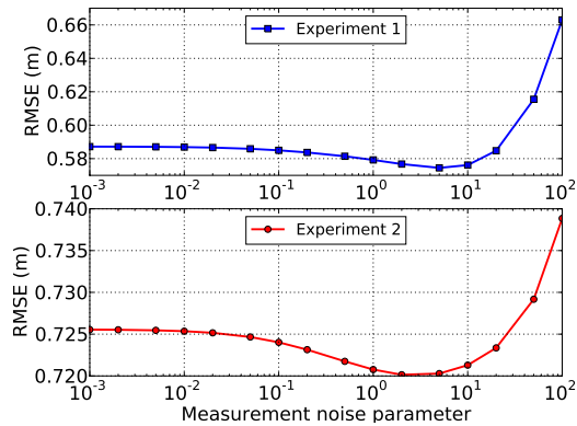
Fig. 14: Tracking RMSE vs. measurement noise parameter \sigma_v^2 .
