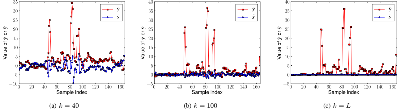
Fig. 3: Effect of principal component number, k , on noise reduction. As k increases, more of the measurement on link l = 588 is attributed to noise, until at k = L , all of the measurement is considered to be noise.
