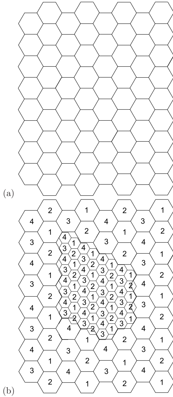
Figure 2: (a) 68 macrocells vs. (b) 53 macrocells plus 57 microcells.
